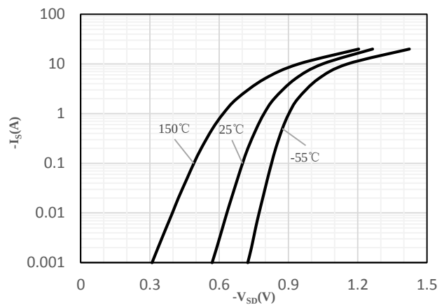
Fig 4 Body-Diode Characteristics
